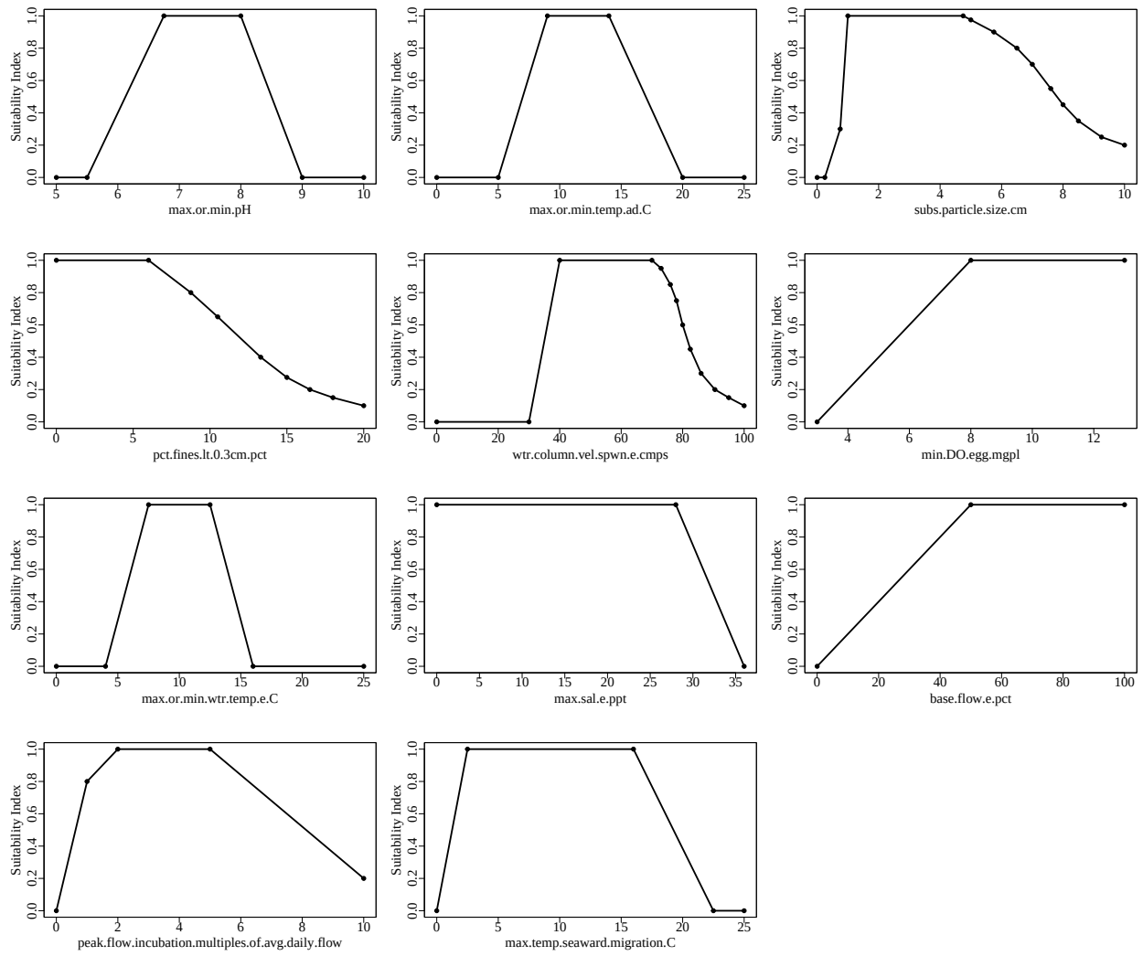
Figure 1. Suitability index graphs for variables included in the pinksalmonLimit model in ecoREST.
